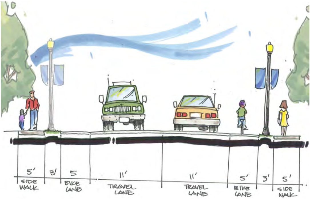
6th Street Corridor Concept A Section
