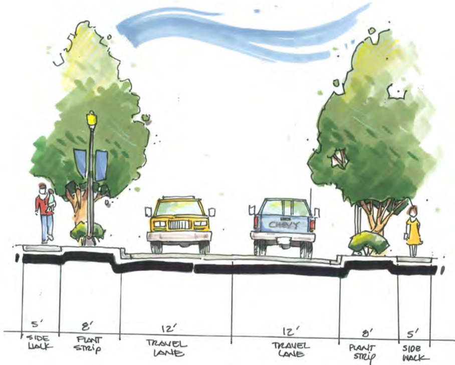
6th Street Corridor Concept B Section
